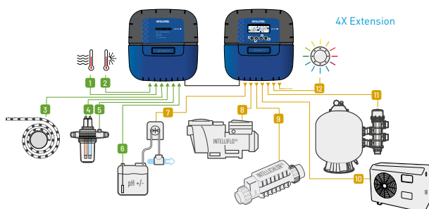
INTELLIPOOL pH
