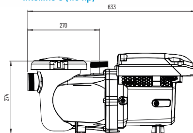
Intelliflo 3 (1.5 hp)
