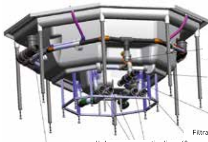
Water connection from gutter to the water tank - 110mm
